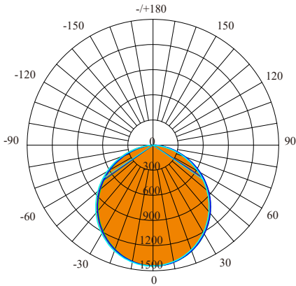
4"/ Diffuser / 3500K
