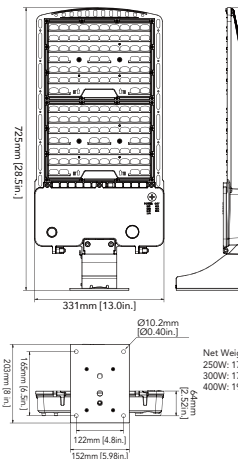
250W/300W/400W (Wall Mount)
