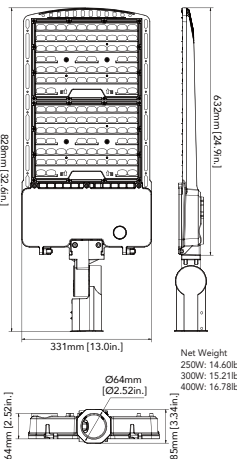
250W/300W/400W (Slipfitter Mount)
