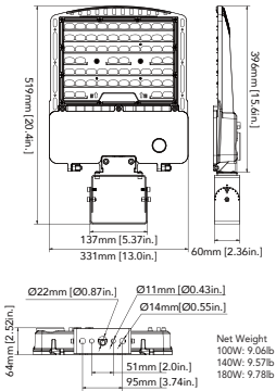
100W/140W/180W (Yoke Mount)
