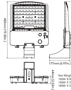
100W/140W/180W (Pole Mount)
