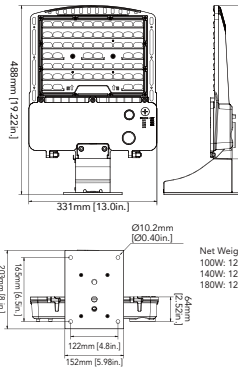
100W/140W/180W (Wall Mount)
