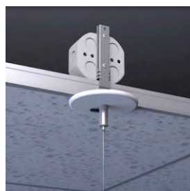
9/16" Flat Ceiling
